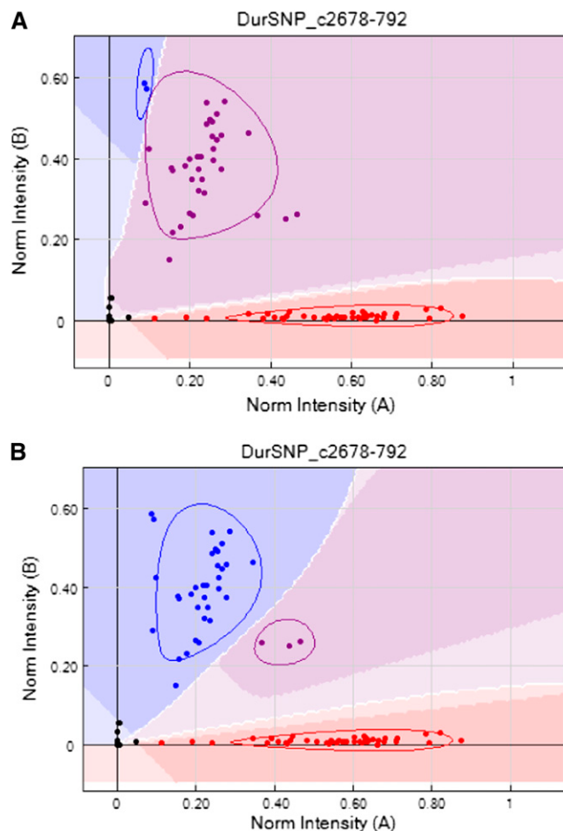
Figure 3 An example of a plot of signal intensities from SNP assay on the tetraploid population using default parameters (A) and after manual correction (B). Points in red and blue are called as homozygotes; points in purple are heterozygotes. Note how genotype calling using default parameters falsely assigns one of the homozygous genotypes as heterozygous.
